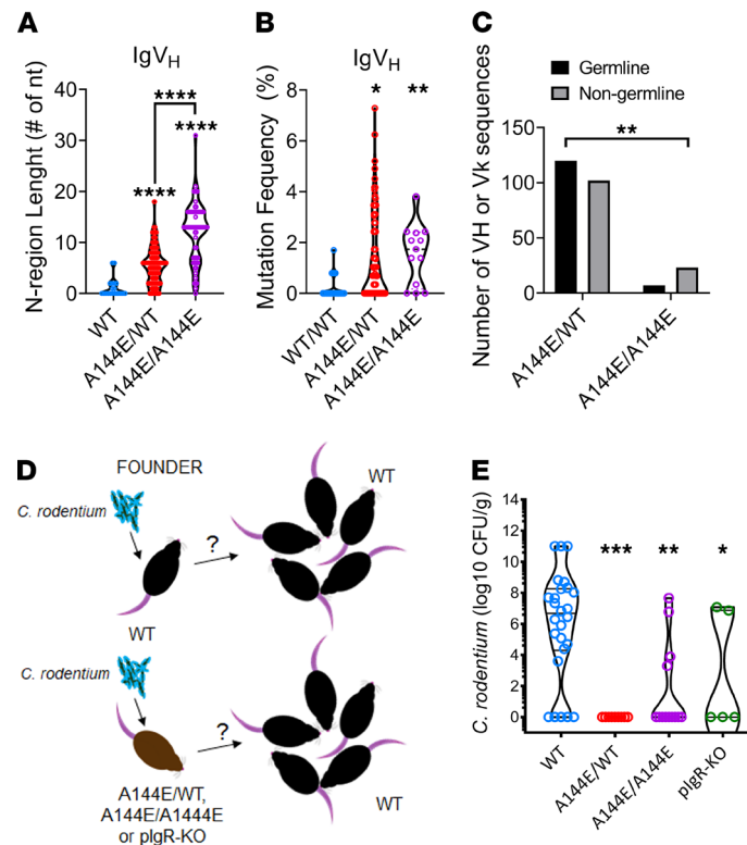
Figure 4. IgA sequences from sorted C. rodentium -bound IgA + B cells of C57BL/6 and Tnfrsf13b mutant mice have distinct properties and determine C. rodentium spreading. Single IgA + GFP- C. rodentium -bound B cells were sorted from the Peyer's patches of infected C57BL/6, A144E/WT, or A144E/A144E mice 14 days following primary infection (A–C) (See also Supplemental Figure 5 and Supplemental Tables 1–6). IgA H+L sequences were obtained from cDNA by PCR followed by Sanger sequencing or by next generation sequencing of barcoded single cell barcoded cDNA libraries. (A) Graphs compare the lengths of the N regions (number of nts) of CDR3 regions (in amino acids) of HC IgA sequences obtained from C57BL/6 A144E/WT or A144E/A144E mice. The Kruskal-Wallis test followed by Dunn's multiple comparisons test yielded P < 0.0001 in comparison of the N region lengths in mutant mice with those in WT mice. (B) Graphs depict the frequencies (%) of mutated nts in VH or Vk exons relative to their closest germline in HC sequences obtained from C57BL/6, A144E/WT, or A144E/A144E mice. The Kruskal-Wallis test followed by Dunn's multiple comparisons test yielded P < 0.0001 in comparison of the N region lengths in mutant mice with those in WT mice, and yielded P = 0.0094 or P = 0.0195 in comparisons of the frequencies of VH gene mutations in A144E/A144E mutants or A144E/WT mice, to those in WT mice, respectively. (C) Contingency analysis of frequency of germline C. rodentium binding IgA, VH, and Vk sequences obtained from A144E/WT or A144E/A144E mice. The \chi^2 test yielded a P = 0.016 , indicating that germline sequences are rarer in A144E/A144E mice compared with A144E/WT mice. (D) Schematic of experimental protocol. Founder mice are either C57BL/6, Tnfrsf13b mutant mice, or pIgR-KO mice. Two founder mice were cohoused with 3 C57BL/6 mice/cage. Only founders were inoculated with low virulence 10^8 C. rodentium . CFUs were counted on not primarily infected mice 7 days after infection. (E) Graph depicts CFU/g feces in mice not primarily infected according to the strain of the inoculated founders (depicted in the x axis). Comparisons were by Kruskal-Wallis tests followed by Dunn's multiple comparison tests. The Kruskal-Wallis test yielded P < 0.0001 ; Dunn's multiple comparison tests to WT yielded *P = 0.0111 , **P = 0.0060 , ***P = 0.0004 , ****P < 0.0001 .
