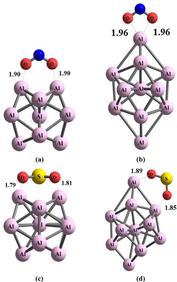
Fig. 3 This figure aims to explain the geometric arrangements of (a) NO 2 @Al 13 , (b) NO 2 @Al 15 , (c) SO 2 @Al 13 , and (d) SO 2 @Al 15 using the optimization method \omega B97XD/Def2-svp. The visual representation displays measurements in Å.
