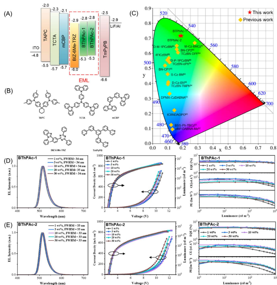
Fig. 5 (A) Device configuration for BThPac-1 and BThPac-2 . (B) Chemical structures of materials used for the devices. (C) CIE coordinates for BThPac-1 , BThPac-2 and reported aggregation-resistant MR-TADF emitters at high doping concentrations (>15 wt%) (Table S7†). (D and E) OLED device performance for BThPac-1 and BThPac-2 .
