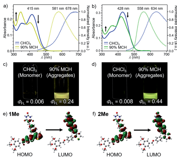
Fig. 2 (a) and (b) UV/Vis absorption (left axis) and fluorescence spectra (right axis, excited at 377 nm for 1 and 392 nm for 2 ) of (a) 1 and (b) 2 in MCH/ \text{CHCl}_3 mixture (MCH fraction = 0% and 90%) ( c = 100 \mu\text{M} ). (c) and (d) Photographs of (c) 1 and (d) 2 in \text{CHCl}_3 (left) and 90 : 10 MCH/ \text{CHCl}_3 (v/v) mixture (right) under 365 nm light illumination ( c = 100 \mu\text{M} ). (e) and (f) Molecular orbitals of the S_0 \rightarrow S_1 transition for model compounds (e) 1Me and (f) 2Me (see ESI † ) calculated at the TD-CAM-B3LYP/6-31+G(d,p) level of theory. The molecular structures of 1Me and 2Me were optimized by DFT calculation at the CAM-B3LYP/6-31+G(d,p) level of theory. For all calculations, dodecyl groups were replaced with methyl groups.
