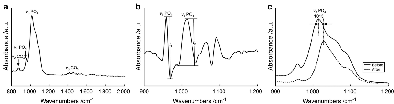
Figure 1 Methods for quantifying the degree of erosion using ATR-FTIR spectroscopy. (a) Baseline-corrected IR spectra in the region of 800–2 000 cm -1 . (b) The peak-to-peak measurement technique applied to spectra that were initially second-derivative transformed and then multiplied by -1 . The ratio of the height of \nu_3 PO 4 ( l_2 ) to that of \nu_1 PO 4 ( l_1 ) was calculated (Method 1). (c) A shift of the \nu_3 PO 4 peak ( \sim 1\ 015 cm -1 ) to a higher wavenumber after erosion treatment was investigated (Method 2). ATR-FITR, attenuated total reflection Fourier transform infrared; a.u., arbitrary unit.
