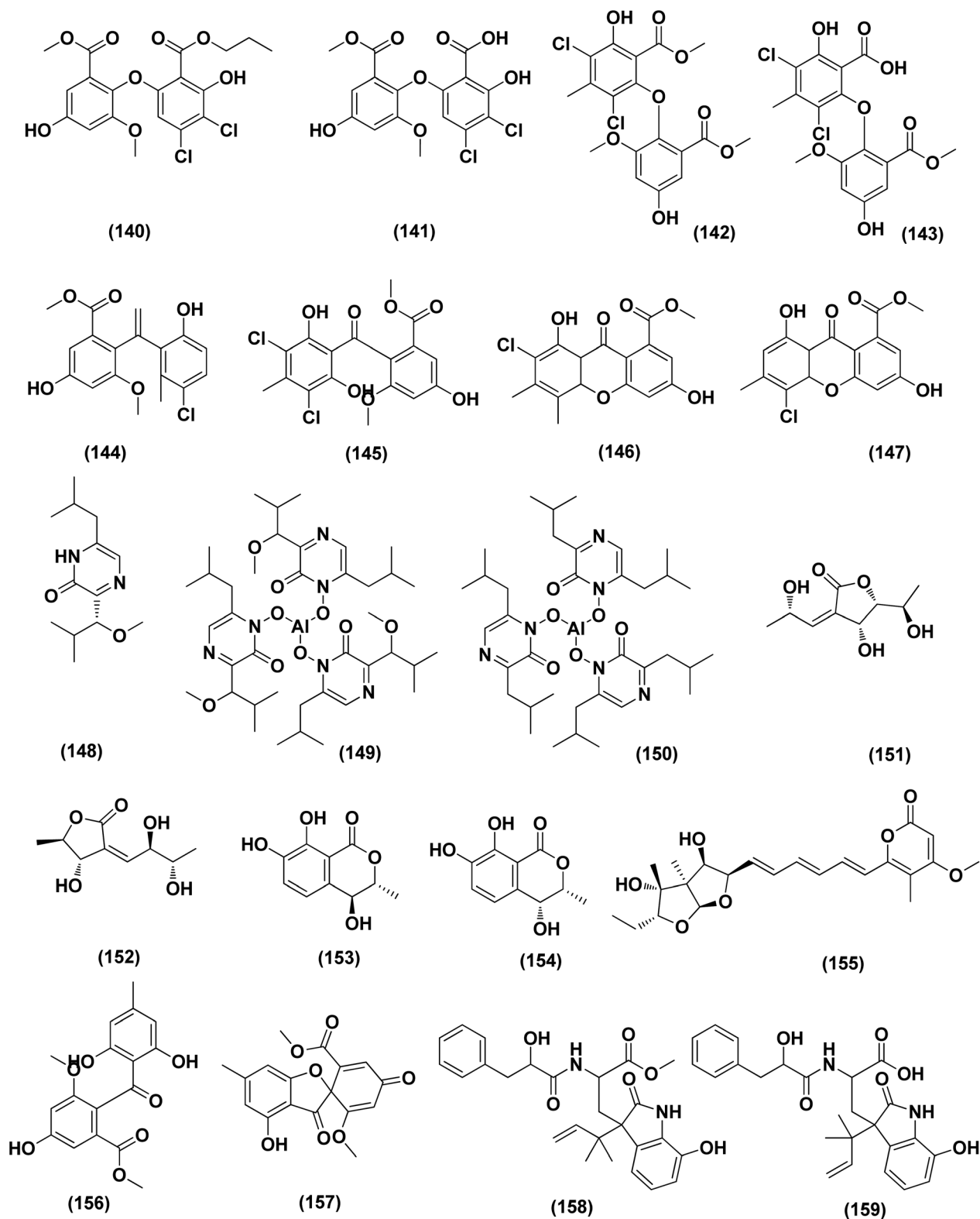
Fig. 9 Chemical structure of compounds 140–159.
