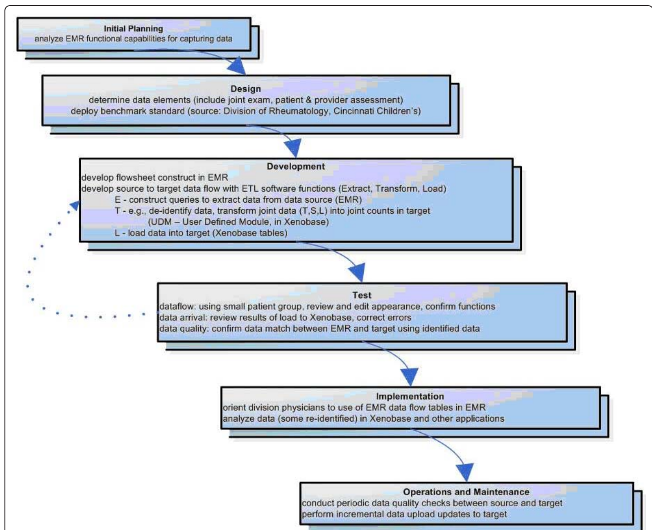
Figure 2 System Development Lifecycle. See Methods for explanation. Development initially affected appearance of the ambulatory EMR by adding forms for entry of specific values for the joint examination, physician and patient global assessment, and patient pain score. The ETL (extract, transform, load) process was implemented external to both the EMR source and analytic software target.
