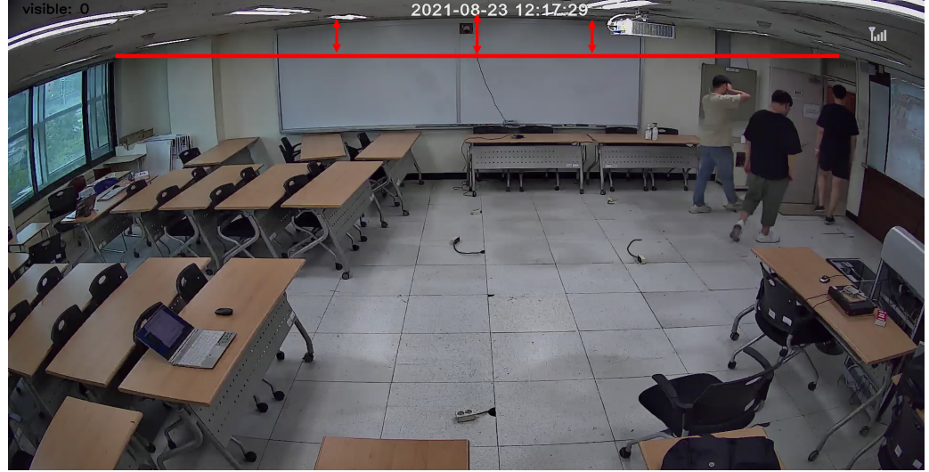
Figure 2. Barrel distortion commonly observed in commercial cameras.
