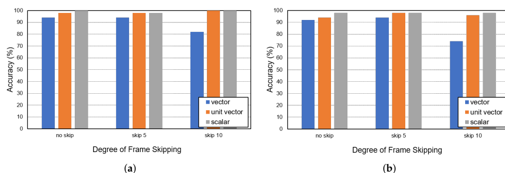
Figure 8. Global ID-matching accuracy with (a) 3 cameras (cameras 1, 2, and 3), and (b) 4 cameras.
