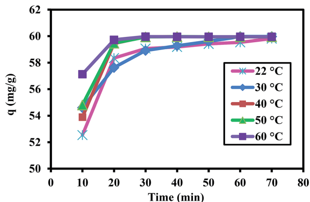
Fig. 7 q vs. time for Cr(vi) concentration of 60 \text{ mg L}^{-1} at pH 2 at different temperatures.
