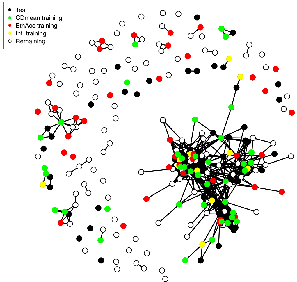
Fig 4. Network representation to highlight the differences in optimized training sets obtained with EthAcc and CDmean as optimization criteria. The data involve a test set of the Flint panel for the DM_Yield trait. This test set had the accuracy of 0.07 and 0.76 when we used as training sets those optimized by CDmean and EthAcc, respectively. The network representation is based on VanRanderen's kinship matrix containing 25 682 SNPs subject to a threshold equal to 0.77 (i.e., individuals were linked in the network if their kinship coefficient was greater than 0.77). Individuals belonging to the test set, the training set optimized via EthAcc, the training set optimized via CDmean, the intersection of the two training sets, and the remaining set are black, red, green, yellow, and white circles, respectively.
