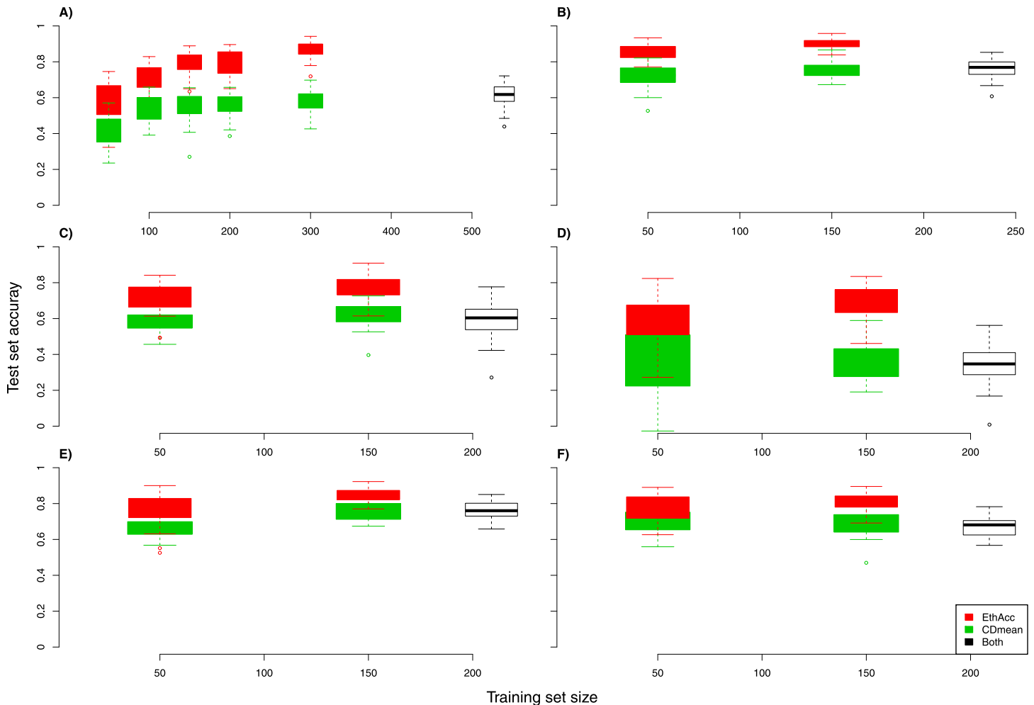
Fig 3. A significant increase in the TS accuracy produced by training set optimization with EthAcc compared to CDmean for several training set sizes and different datasets. The optimal (but inaccessible without test phenotypes) training set is the starting set of the optimization process. The black boxplot corresponds to the largest training set. A) WSY within sugar beet Panel_A. B) DOY for wheat. C) DM_Yield within the Dent panel. D) DM_Yield within the Flint panel. E) Tass_GDD6 within the Dent panel. F) Tass_GDD6 within the Flint panel. Boxplots were constructed from 30 random test sets representing 20% of the whole panel.
