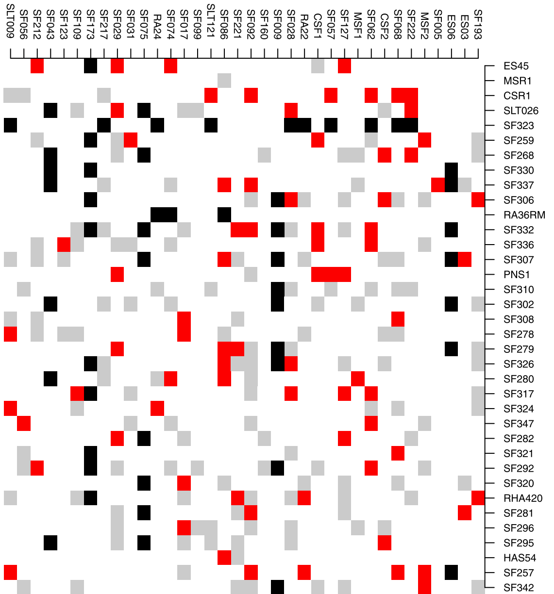
Fig 2. SUNRISE hybrids obtained from 36 maintainer lines (females, rows) crossed to 36 restorer lines (males, columns). Parental lines are arranged according to the hierarchical clustering based on VanRaden's kinship matrices. Black squares indicate the 54 T0 or T1 hybrids in the test set, red squares are the 77 training individuals, and grey squares are hybrids that were among candidates but were not chosen to be in the training set.
