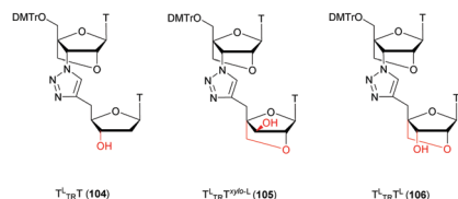
Fig. 18 Chemical structures of T_{-Tr}^L T ( 104 ), T_{-Tr}^L T^{xylo-L} ( 105 ) and T_{-Tr}^L T^L ( 106 ) TR-LNA-dithymidines.
