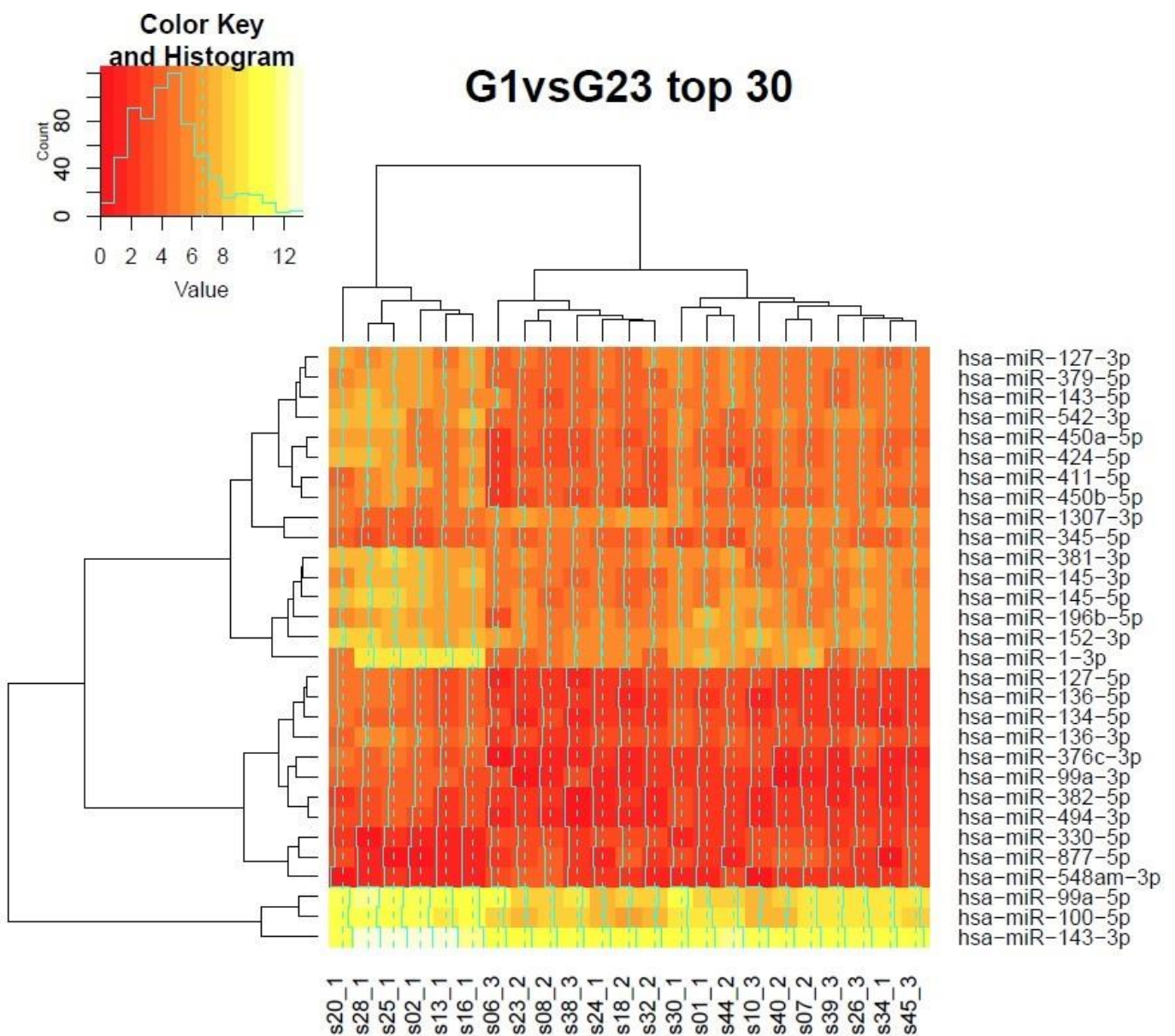
Figure 3. Clustering of the top 30 differentially expressed miRNAs of G1 patients vs. collected-together patients with G2 and G3 grade. Value = miRNA gene reads. At the bottom of the picture is the sample’s name with grade indication.
