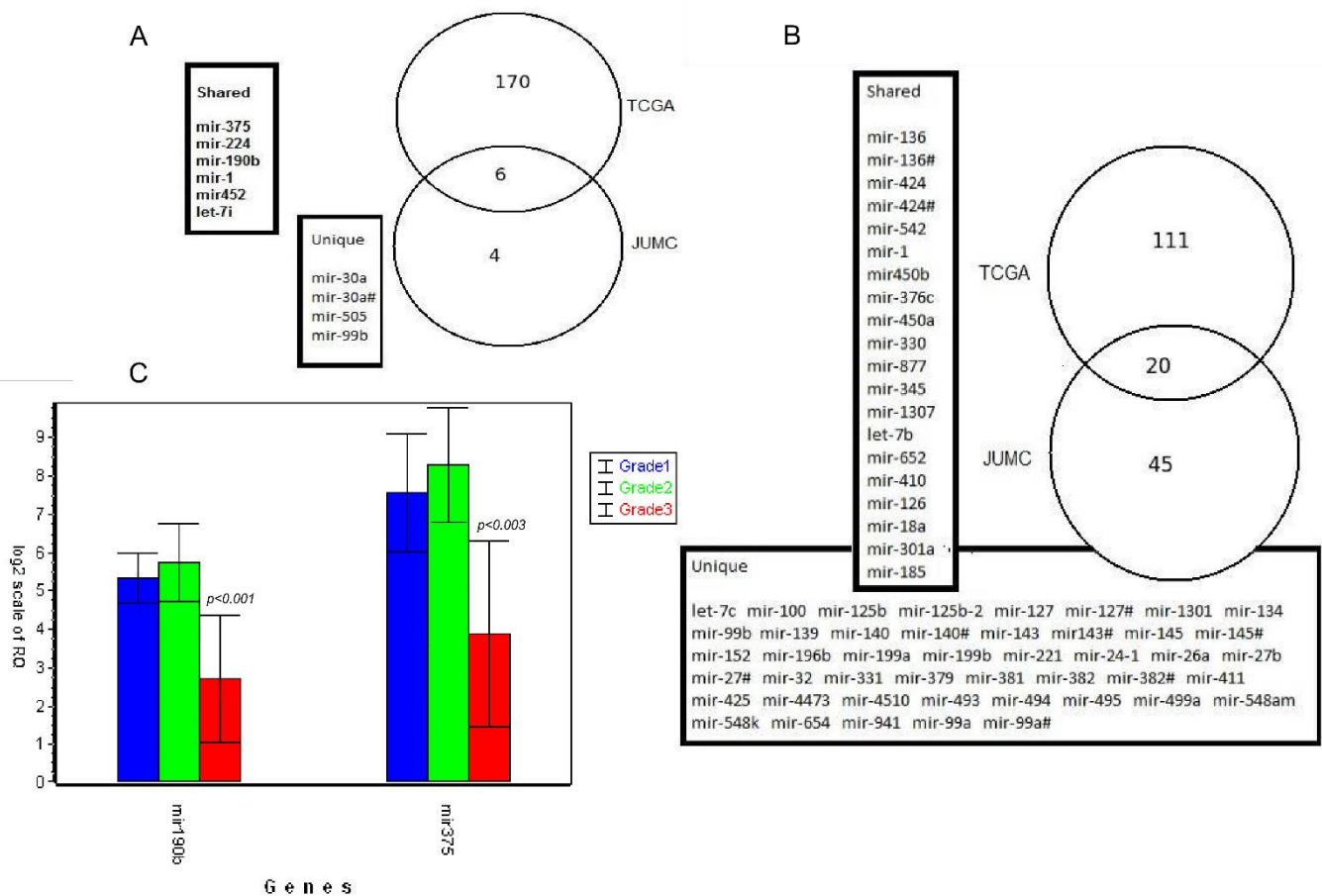
Figure 2. Overlapping miRNA genes between studied cohort (JUMC) and data collected by the Cancer Genome Atlas (TCGA) cohort. Venn diagrams shows the number of differentially expressed genes between G1 + G2 vs. G3 (A) and G1 vs. G2 + G3 (B). Unique and shared miRNA are listed in frames. (C) shows qPCR relative expression results of miR-190b and miR-375. JUMC, Jagiellonian University Medical College; studied cohort, TCGA; the Cancer Genome Atlas; blue bar, grade 1; green bar, grade 2; red bar, grade 3.
