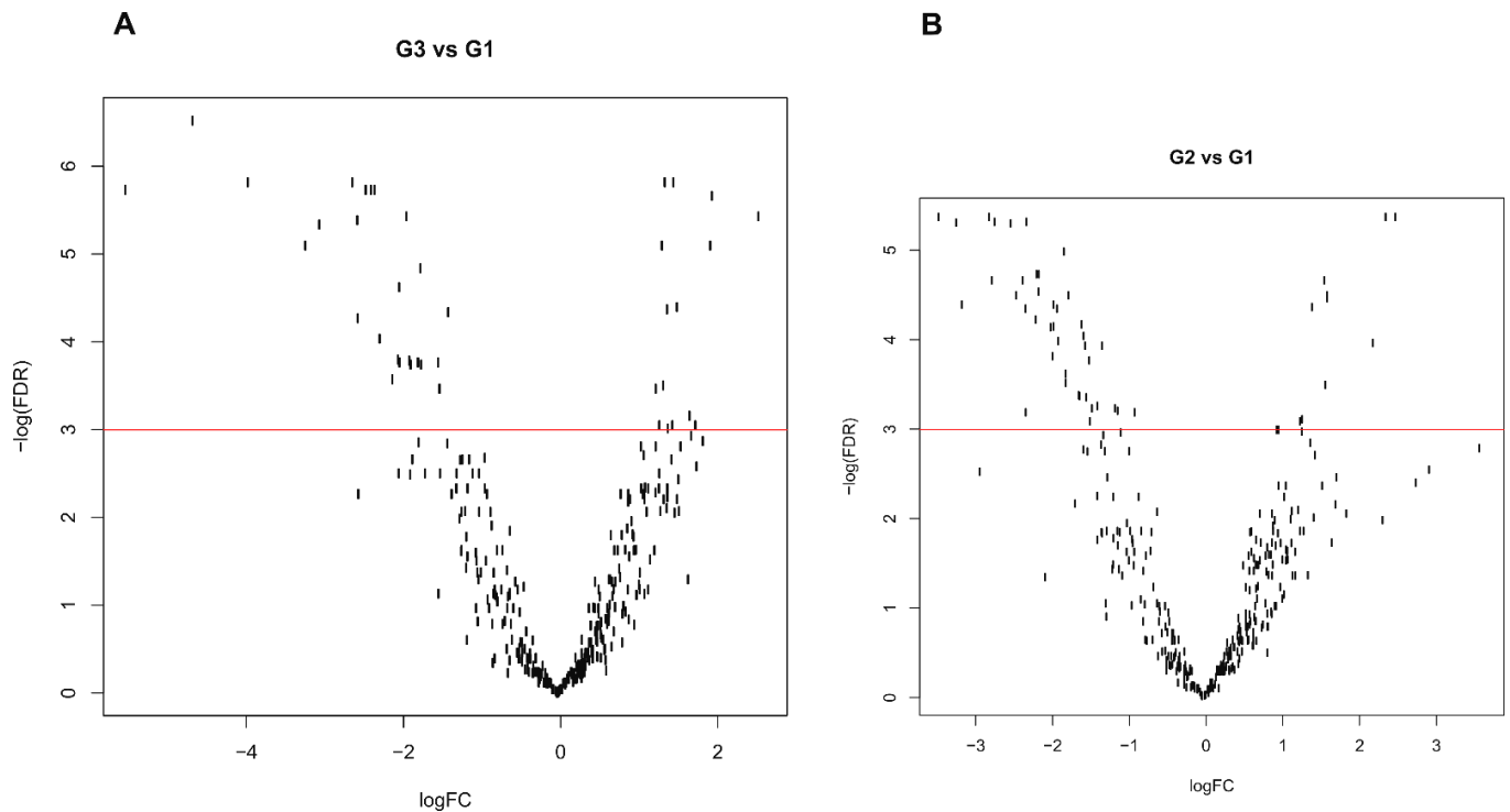
Figure 1. Volcano plots of differential expressed genes (DEG) between individual grades. (A) DEG between grade 3 and grade 1 samples. (B) DEG between grade 2 and grade 1 samples. X axis, logarithmic fold change value (logFC) and Y axis, negative logarithmic value of false discovery rate ( -\log(\text{FDR}) ). Each dot represents an individual miRNA transcript.
