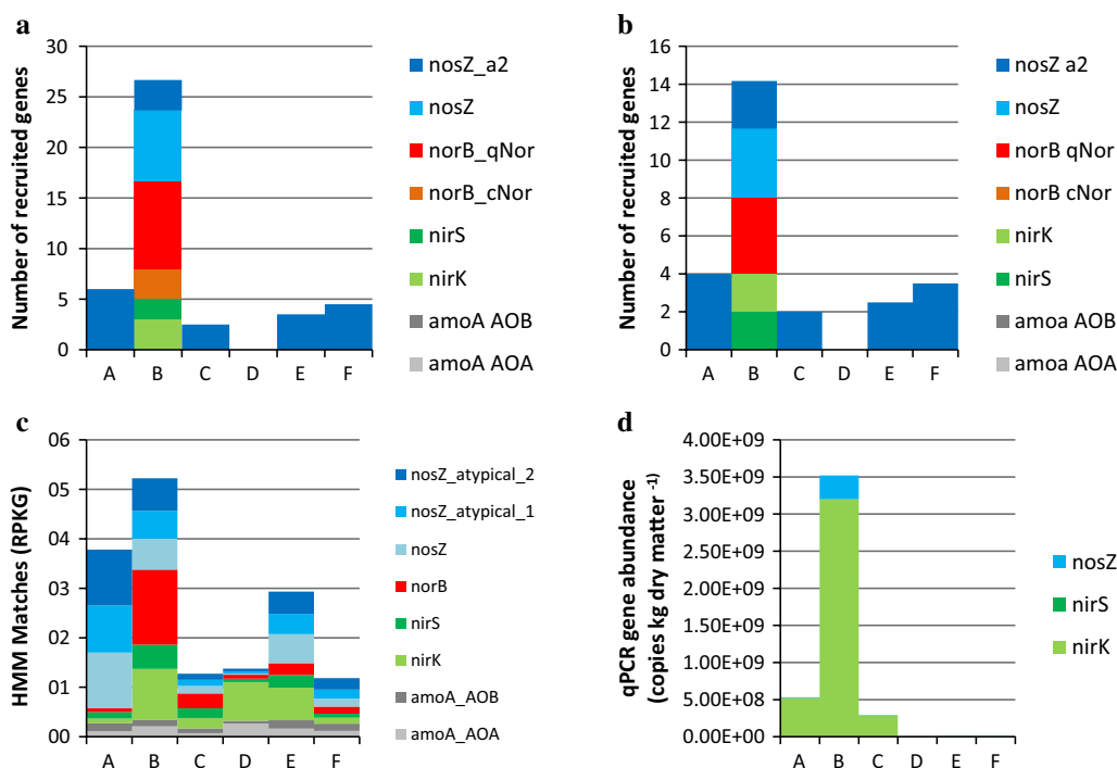
Fig. 3 Putative gene abundances in the vinasse metagenomes. Partial gene fragments were recruited from the vinasse metagenomes using megagta on (a) all reads and (b) rarified reads. In parallel, vinasse metagenomes were compared to profile HMMs and the number of matches was normalized to (c) reads per kilobase per genome equivalent (RPKG). In (d) the gene copy numbers from real-time PCR of the nosZ , nirS and nirK genes are depicted. Note that no qPCR of the norB gene was made
