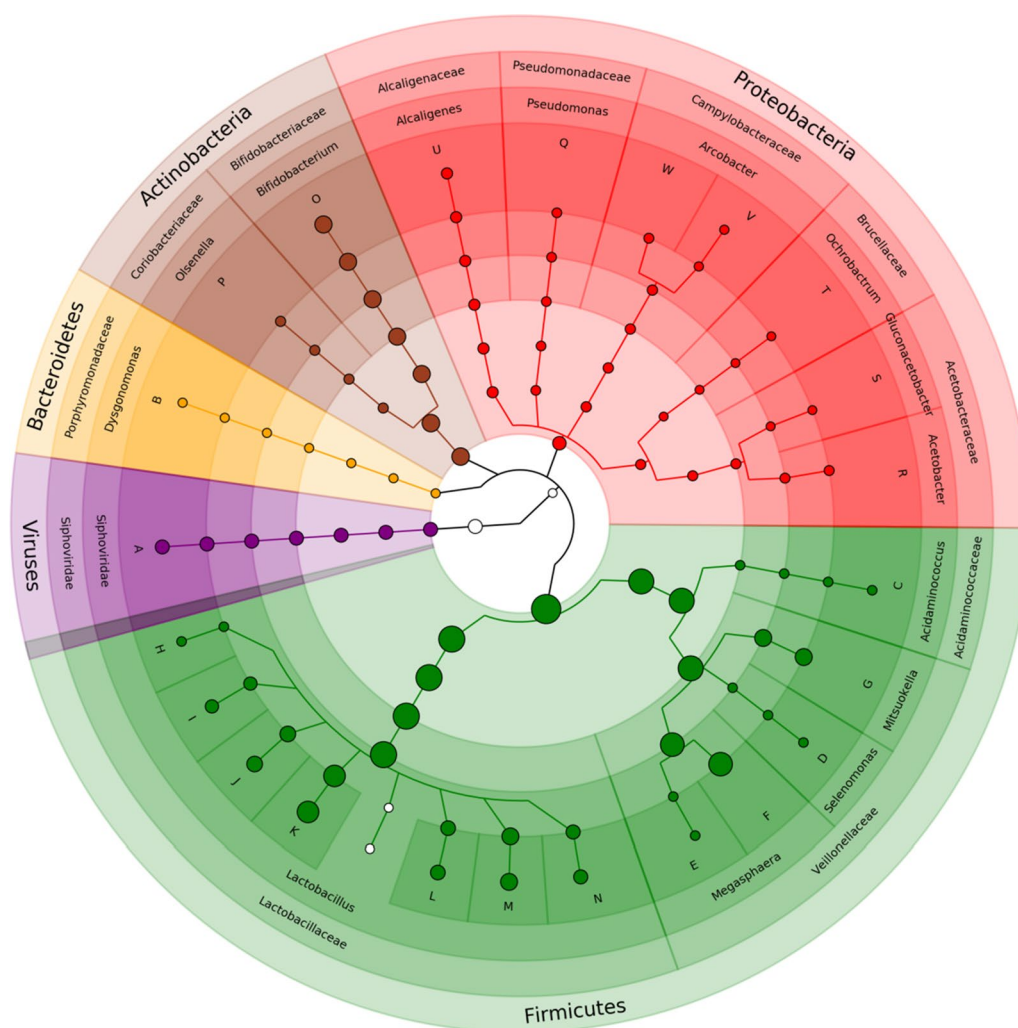
Fig. 1 Average abundance of taxa in the vinasse samples. The metagenomes were analyzed using metaphlan2 and visualized with GraPhlAn. Node sizes correspond to average relative abundance across the vinasse metagenomes while colors correspond to phylum. Species are noted with letters: A = Lactobacillus phage Lc Nu, B = D. mossii , C = A. intestini , D = S. bovis , E = M. elsdenii , F = Megasphaera unclassified, G = Mitsuokella unclassified, H = L. salivarius , I = L. equicursoris , J = L. delbrueckii , K = L. amylovorus , L = L. mucosae , M = L. fermentum , N = L. vini , O = B. thermophilum , P = Olsenella unclassified, Q = Pseudomonas unclassified, R = Acetobacter unclassified, S = Gluconacetobacter unclassified, T = Ochrobactrum unclassified, U = A. faecalis , V = A. butzleri and W = Arcobacter unclassified
