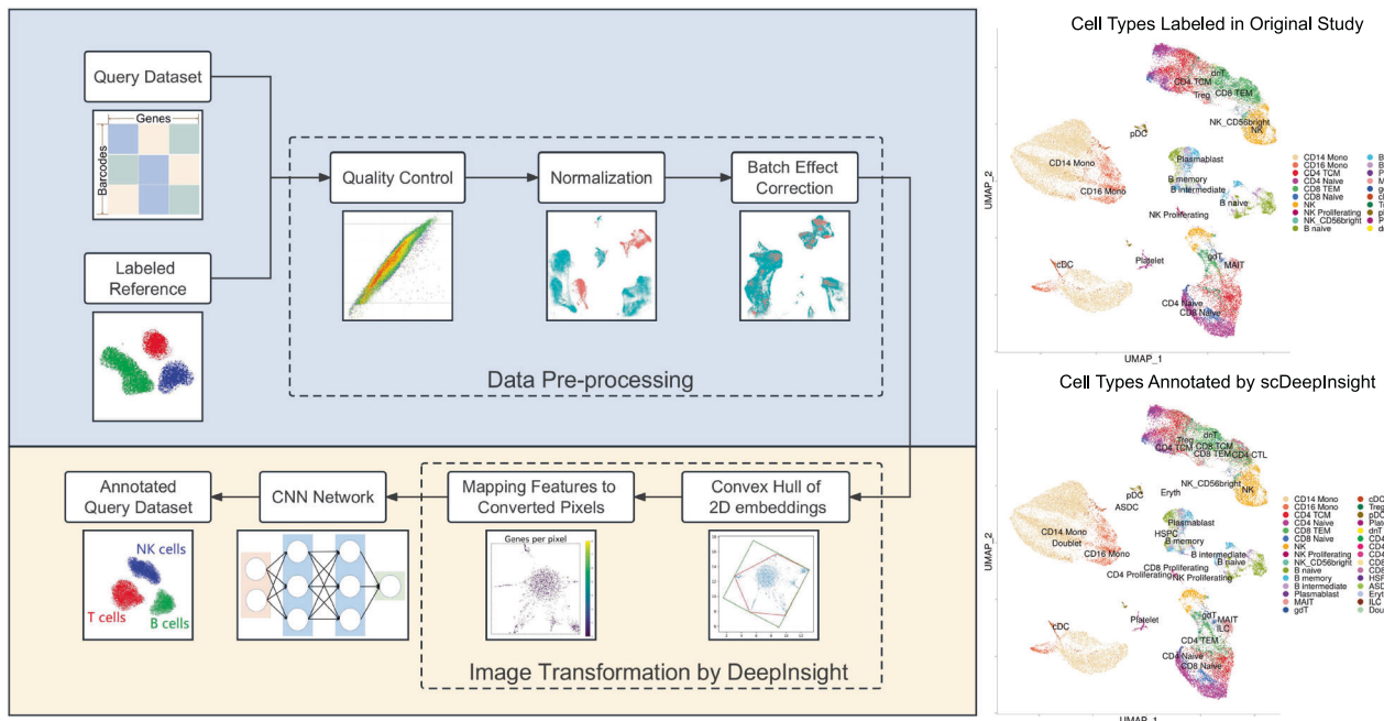
Fig. 6 On the left, scDeepInsight's workflow progresses from inputting the molecular identifier to generating cell annotations. After processing a reference dataset and query data, they are translated into 2D images, which are used for training the CNN model. Notably, only the reference data trains the model, while the query set is classified. For future query sets, the existing model can be directly applied without new training. On the right, a UMAP visualization of a query dataset shows labeled cell types from the initial study, contrasted with a UMAP colored by scDeepInsight's predictions. (From Jia et al. [21] under creative commons license.)
