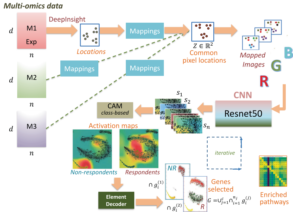
Fig. 5 Overview of the DeepInsight-3D model. Starting from the left, multi-omics layers undergo processing via the DeepInsight methodology to identify common pixel locations. Upon mapping omics data, the corresponding images are constructed and then fed into a CNN architecture. Subsequently, CAM is employed to determine activation regions, while the element decoder pinpoints a subset of genes. (From DeepInsight-3D paper [19] under creative commons license.)
