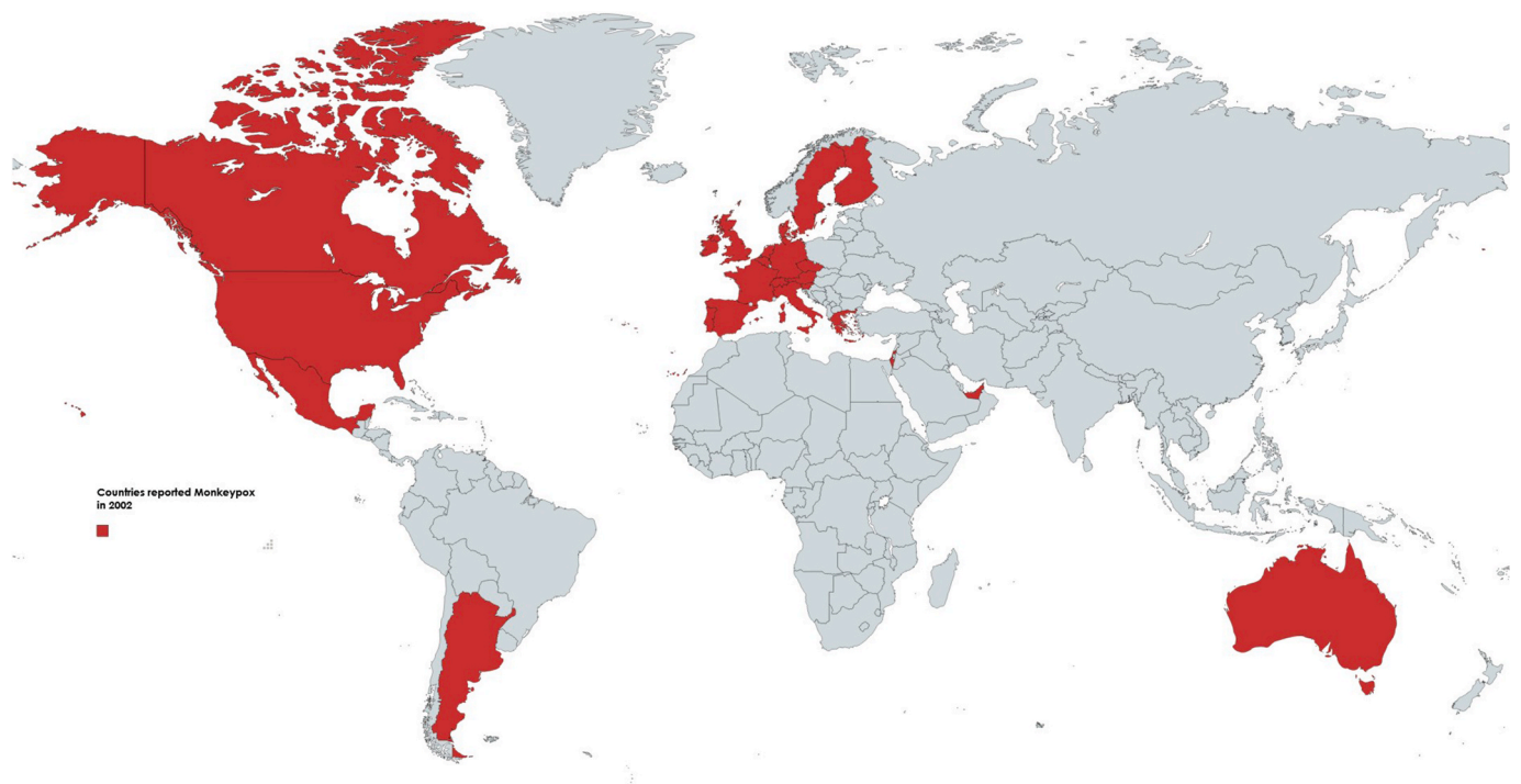
Fig. 1. Geographical distribution of confirmed and suspected cases of monkeypox in non-endemic countries in 2022, up to May 29.
