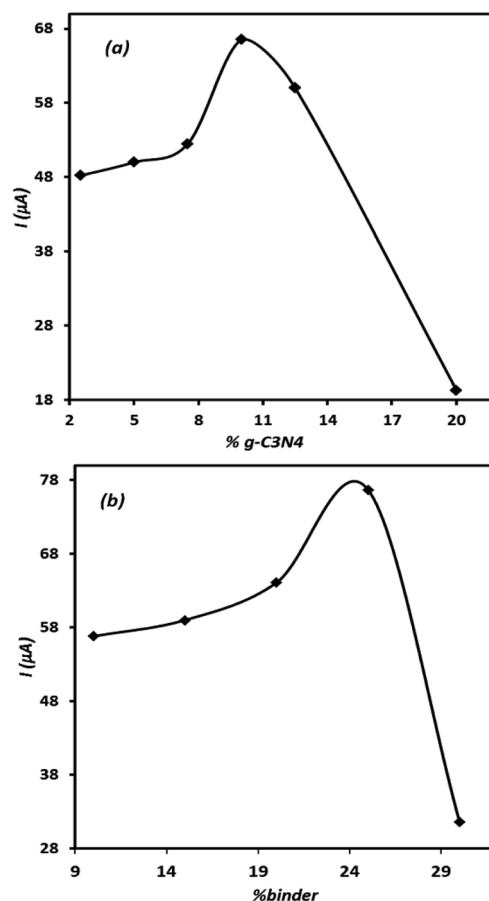
Fig. 5 The effect of g\text{-C}_3\text{N}_4 (a) and binder (b) percent on the electrode response; cyclic voltammetry conditions: [\text{OA}] = 1 \times 10^{-3} \text{ M} in 50.0 \text{ mmol L}^{-1} of ammonium acetate (pH = 6), scan rate = 100 \text{ mV s}^{-1} .
