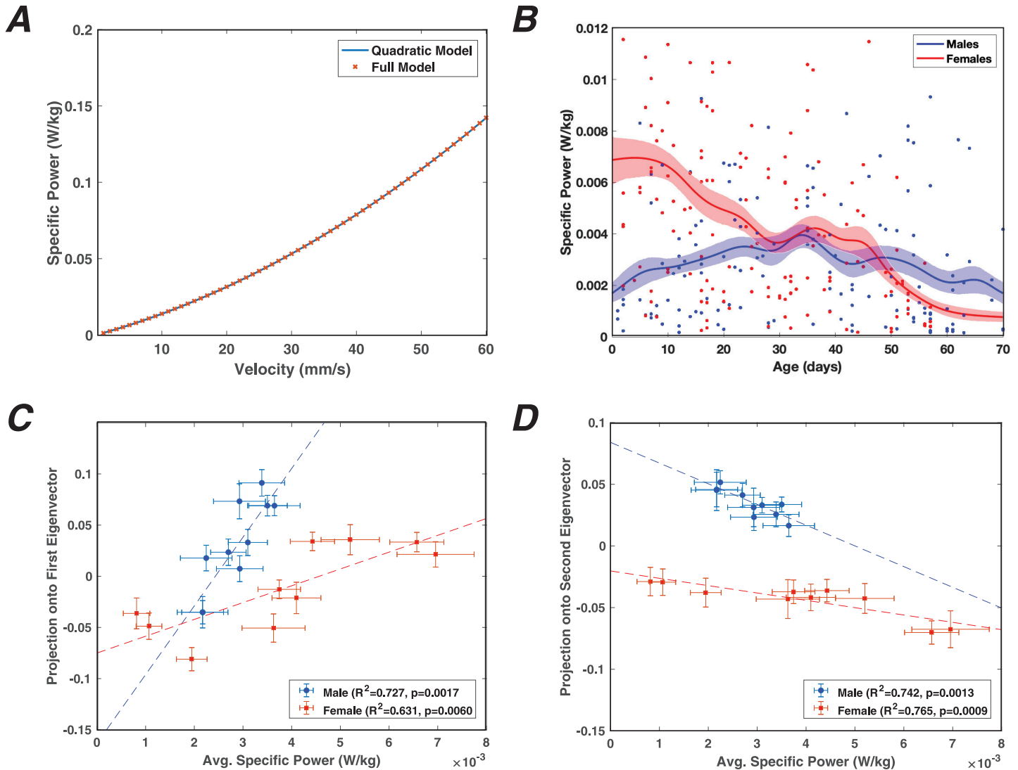
Fig 4. Energy usage predicts aging-specific changes in behavior. (A) Comparison of the quadratic model to the full model of Nishii (2006) to estimate specific power (power per unit mass) of legged locomotion in fruit flies. (B) Specific power as a function of age for male (blue) and female (orange) fruit flies. Each point represents an individual, and the curves are the Gaussian-smoothed means ( \sigma = 3.5 days), with error bars generated in the same manner as Fig 3D. (C) Average projections onto the first eigenmode (Fig 3C (top)) plotted versus the average specific power consumption for both male and female flies. Each point represents the value (plus error bars) from the curves in (B) and Fig 3D (top), each spaced 7 days apart. Dashed lines are the linear fits to the data. (D) Same as (C), but instead using projections onto the second eigenmode (Fig 3C (bottom)). Note that at over 70% of the mean aging-specific variation can be explained using the first two eigenmodes.
