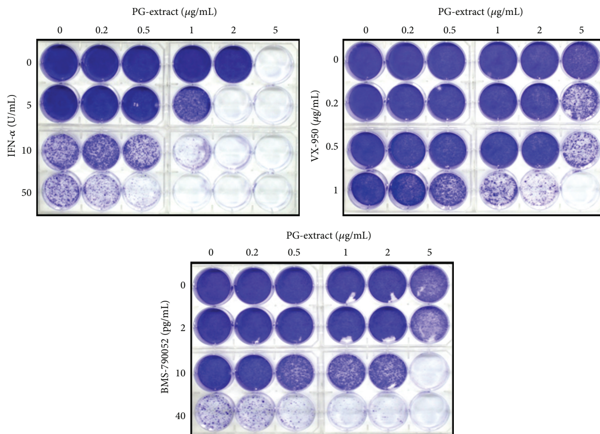
FIGURE 7: PGSM potentiates colony suppression in replicon cells in combination with IFN- \alpha and DAAs. HCV replicon cells were treated with various concentrations of PGSM and IFN- \alpha , PGSM and BMS-790052 (NS5Ai), and PGSM and VX-950 (PI) as indicated. Three weeks after treatment, remaining surviving cells were stained with crystal violet.
