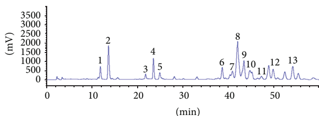
FIGURE 2: Representative HPLC/ELSD chromatograms of triterpenoid saponins in PGSM. The numbers indicate each triterpenoid saponin: 1, deapi-platycode E; 2, platycoside E; 3, deapi-platycode D 3 ; 4, platycodin D 3 ; 5, platyconic acid A; 6, deapi-platycode D; 7, platycodin D 2 ; 8, platycodin D; 9, polygalacin D; 10, 3''-O-acetylpolygalacin D; 11, platycodin A. 12, deapio-3''-acetyl polygalacin D; 13, 2''-O-acetyl platycodin D.
