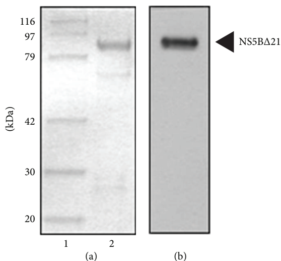
FIGURE 4: Purification of HCV NS5B protein. (a) HCV NS5B protein (1 \mu g) eluted from glutathione sepharose affinity column was subjected to SDS-polyacrylamide gel electrophoresis and visualized by Coomassie Brilliant Blue R-250; (b) NS5B protein purified from figure legend to A was immunoblotted with an anti-NS5B monoclonal antibody and visualized with the enhanced chemiluminescence detection. The arrowhead indicates the NS5B protein.
