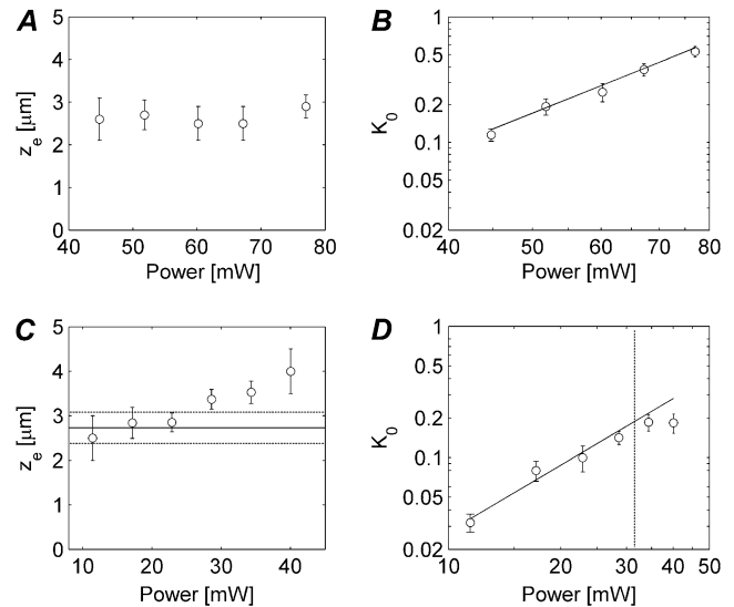
FIGURE 4 (A) Two-photon FRAP experiments were performed on FD500 in an 85% (w/w) glycerol solution by bleaching a disk of 3 \mu\text{m} in radius with different laser powers to evaluate the axial extension z_e of the effective photobleaching PSF. The axial bleaching resolution was determined by fitting of the two-photon disk FRAP model to the experimental recovery curves. Every data point is the average of 10 measurements. The error bars are the corresponding standard deviations (SDs). (B) The corresponding K_0 values are shown as a function of the bleaching laser power in a log-log plot. The slope of the linear fit is 2.7. (C) The same measurement was performed on paGFP in a solution containing 56% (w/w) of sucrose. The horizontal solid line represents the average of the z_e values corresponding to a laser power \leq 25 mW. The dashed lines indicate the corresponding SD. (D) A log-log plot of K_0 as a function of the photoactivation laser power is shown. The solid line is a linear fit to the data at the left of the vertical dashed line, having a slope of 1.8.
