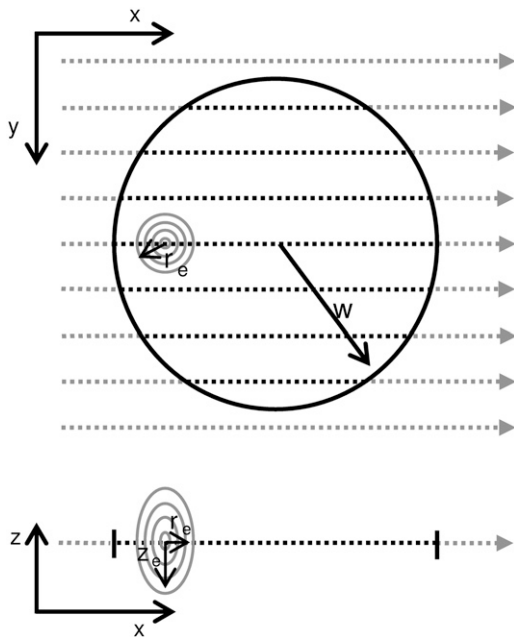
FIGURE 1 Schematic representation of the bleaching phase of a two-photon FRAP measurement. The bleaching illumination distribution I_b(x,y,z) scans line by line the selected circular region of radius w . A high laser power is delivered on the sample when the system is scanning the inner part of the circle (dashed lines), inducing the photobleaching/photoactivation of the fluorescent molecules. An x,z view of the scanning process is also shown, where r_e and z_e are the axial and radial 1/e^2 extensions of the Gaussian bleaching illumination distribution.
