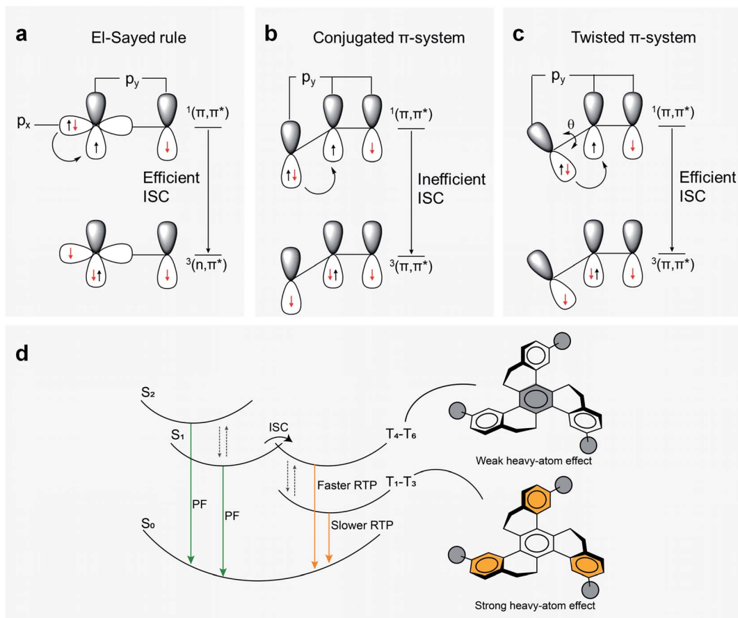
Fig. 7 Possible ISC pathways and emission mechanism. (a) Representation of transitions from ^1(\pi, \pi^*) to ^3(n, \pi^*) states, in agreement with El-Sayed's rule, from p_x to p_y orbitals that efficiently overlap under SOC, inducing an efficient ISC mechanism. ^1(n, \pi^*) to ^3(\pi, \pi^*) transitions are likewise allowed by El-Sayed's rule. (b) By contrast, ISC from ^1(\pi, \pi^*) to ^3(\pi, \pi^*) (or from ^1(n, \pi^*) to ^3(n, \pi^*) ) is disfavored in a planar aromatic system because orbital overlap is poor and SOC is inefficient. (c) In a twisted aromatic molecule, a transition between two (\pi, \pi^*) states comes with nonvanishing SOC matrix elements, allowing an efficient ISC. (d) Proposed mechanism for RTP in HTX and its halogenated derivatives. After excitation, dual PF deactivates the S_1 and S_2 excited states to the ground state ( S_0 ) (Fig. S8–S12†). Considering that k_{PF}(S_2) \gg k_{ISC} , the excited molecule may also transform from S_1 to T_1 through ISC, enabling a faster Ph decay and the slower Ph with \mu\text{s} to \text{ms} lifetimes at RT. Due to the presence of low-lying excited triplet states well below S_1 , the HAE enhances only slightly k_{ISC} , whereas k_{Ph} is strongly affected.
