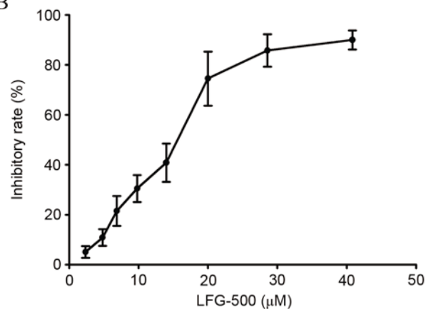
Figure 1. Chemical structure and inhibitory effects of LFG-500 on the growth of SKOV3 cells. (A) Chemical structure of LFG-500 ( C_{30}H_{32}N_2O_5 ). (B) Inhibitory effects of LFG-500 on the growth of SKOV3 cells after 24 h, as measured by the MTT assay. LFG-500, synthetic flavonoid compound; SKOV3; human ovarian carcinoma cell line.
