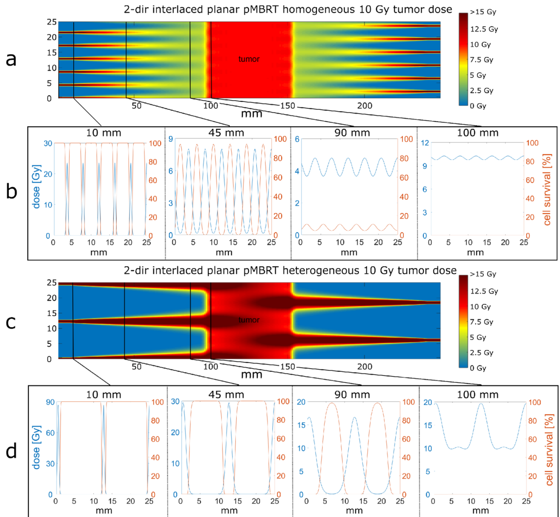
Figure 2. Dose maps of 2-dir interlaced planar minibeams (cf. Fig. 1c) with homogeneous (a) and heterogeneous (c) tumor dose. The dose is color-coded with saturation at 15 Gy. The cross-section of dose and the local clonogenic cell survival at 10, 45, 90 and 100 mm depth are shown for homogeneous (b) and heterogeneous (d) tumor irradiation with 10 Gy mean or minimum tumor dose, respectively. Heterogeneous tumor irradiation is described in section III.B.
