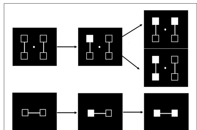
FIGURE 5 | Illustration of the successive events in the simultaneity/asynchrony discrimination task in case of an asynchrony (from left to right). When four locations are used (upper row) and the first square is filled in (middle figure in the upper row), there are two possible locations for the second one (figure on the right), and there is thus an uncertainty regarding the location of the second stimulus. The spatial location of the second stimulus is always predictable when only two locations are used (lower row). These two experiments have been
