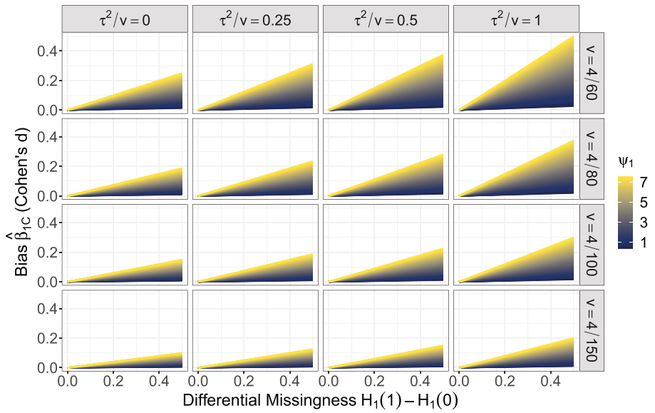
FIGURE 2 The bias of \hat{\beta}_{1C} (y-axis). Each panel corresponds to a given value of residual heterogeneity \tau^2 and estimation error variance v . Within panels, the bias of \hat{\beta}_{1C} is plotted as function of differential missingness rates ( p(R = 0|X = 1) - p(R = 0|X = 0) ), which is analogous to the correlation between the value of X and whether it is observed. Bias is also shown as a function of \psi_1 , which is the relationship between the probability of observing X , and the effect size T . Bias is shown on the scale of Cohen's d and \psi_1 is on the scale of a log-odds ratio [Colour figure can be viewed at wileyonlinelibrary.com ]
