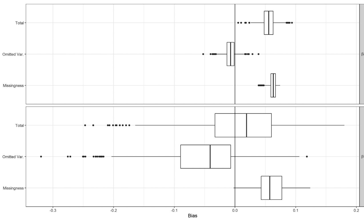
FIGURE 4 Bias in shifting-case analysis (SCA) regression of T_i on X_{i1} . For both the intercept \beta_0 and slope \beta_1 , these boxplots show the total potential bias of the SCA estimators, as well as the omitted variable and missingness bias. Units are shown on the scale of Cohen's d
