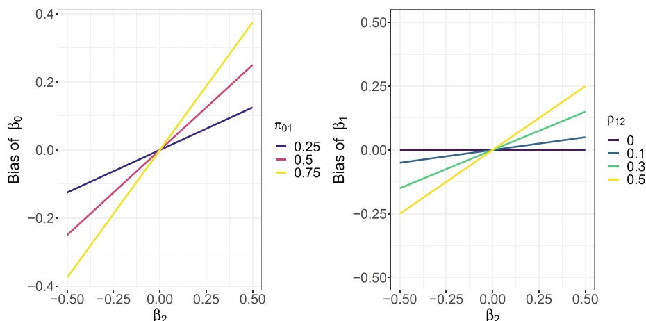
FIGURE 3 The omitted variable bias of \hat{\beta}_{0S} and \hat{\beta}_{1S} for model (27) as a function of the omitted variable coefficient \beta_2 . The bias (y-axis) and \beta_2 (x-axis) are on the scale of Cohen's d . The bias displayed is solely due to omitting X_{i2} from model (27). In the left plot, lines are colored according to \pi_{01} = p(X_{i2} = 1 | X_{i1} = 0) . In the right plot, lines are colored according to \rho_{12} = p(X_{i2} = 1 | X_{i1} = 1) - p(X_{i2} = 1 | X_{i1} = 0) [Colour figure can be viewed at wileyonlinelibrary.com ]
