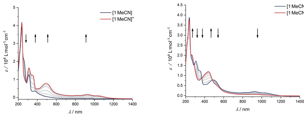
Fig. 4 UV/Vis-SEC of complex [1 \cdot \text{MeCN}] in \text{MeCN}/n\text{-Bu}_4\text{PF}_6 at 293 K. Left: Spectral changes during first oxidation. Right: Spectral changes during second oxidation.
