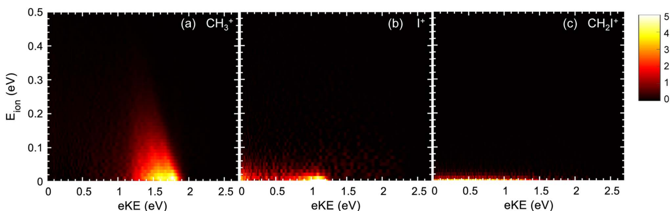
Fig. 2 Electron–ion kinetic energy correlation diagram, E_{\text{ion}} vs. eKE, for (a) (\text{CH}_3^+, e) , (b) (\text{I}^+, e) , and (c) (\text{CH}_2\text{I}^+, e) coincident events following excitation at photon energy 14 eV. The color bar shows the scale (in arbitrary units) for (b) and must be \times 6 for (a) and \times 2 for (c).
