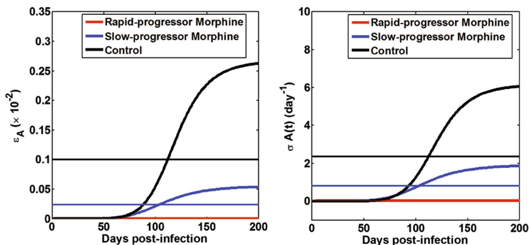
Figure 4. Predicted effects of morphine-altered virus-specific antibody responses on virus neutralization and enhanced virus clearance. The horizontal lines show the mean values of \epsilon_A and \overline{\sigma A(t)} for each group calculated over a period of 200 days post infection using \overline{\epsilon_A} = \frac{1}{200} \int_0^{200} \left( \frac{\eta A(t)}{1 + \eta A(t)} \right) dt and \overline{\sigma A(t)} = \frac{1}{200} \int_0^{200} \sigma A(t) dt . Note that for the rapid-progressor morphine group, we can obtain the analytic solutions as \overline{\epsilon_A} = \frac{\eta a}{1 + \eta a} and \overline{\sigma A(t)} = \sigma a .
