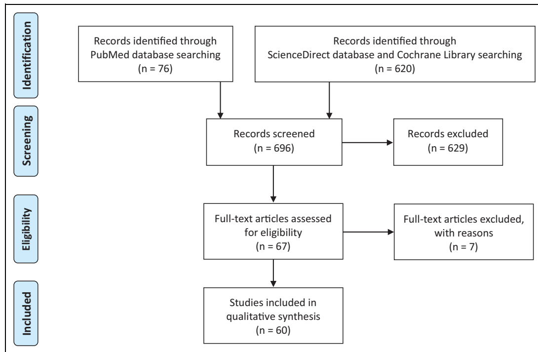
Figure 1. PRISMA flowchart.
