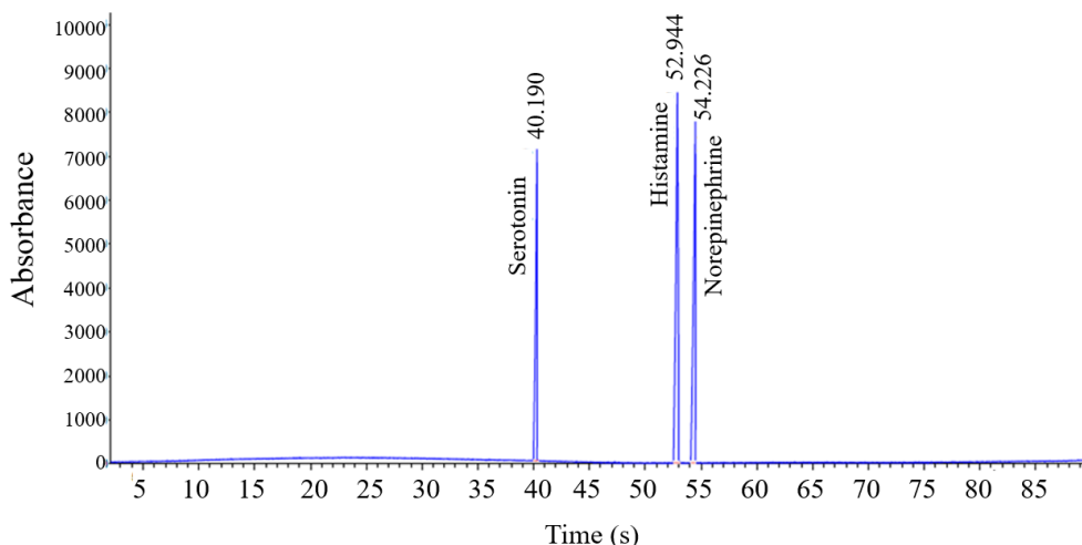
Fig. 2. SIM graph of the real sample Bufo viridis secretion extract in SIM mode (serotonin (30, 42, 204, 58), histamine (82, 30, 54, 41), norepinephrine (111, 65, 93, 139)). SIM, Selected ion monitoring.
