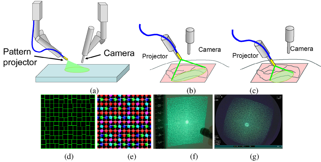
FIGURE 1 (a) Active-stereo 3D scanning system in laparoscopy. (b),(c) Scanning 3D shape by moving the projector and the camera. (d) The projected grid pattern. (e) Code information embedded into the pattern. (f) The pattern illuminated onto a plane. (g) Pattern-illuminated surface captured by the laparoscopic camera.
