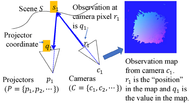
FIGURE 3 Observation model of active stereo systems.
