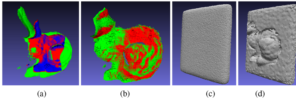
FIGURE 6 Calibration results of simulation data. (a) Shapes before and after single-frame auto-calibration. Colored point clouds are (red) ground-truth shape, (green) before auto-calibration, and (blue) after auto-calibration. The green colored shape reconstructed by un-calibrated parameters was severely distorted, whereas ground-truth shape and auto-calibrated shapes were almost identical. (b) Result of 2-frame calibration, where red points are frame #1 and greens are #2. Note that multiple frames were fit to each other by disambiguation of scale inconsistency by auto-calibration. (c) Initial shape and (d) shape after optimization, showing rabbit-shape is successfully recovered.
