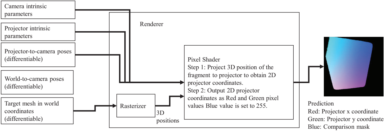
FIGURE 4 Differentiable renderer with differentiable variables of C , P , and S .
