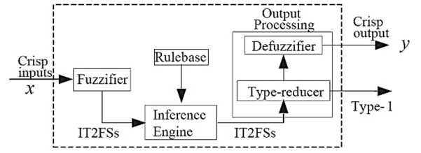
Fig. 3. The structure of the IT2FLS [47].
