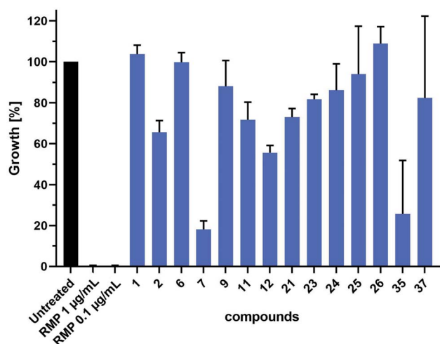
Fig. 6 Head-to-head comparative analysis of the antiTB activity of DCC hits. mCherry-expressing M. tuberculosis H37Rv bacteria were cultured in the absence or presence of DCC hits (16 \mu\text{M} ) or rifampicin (RMP, pos. ctrl). Shown are data of two independent experiments performed in triplicates.
