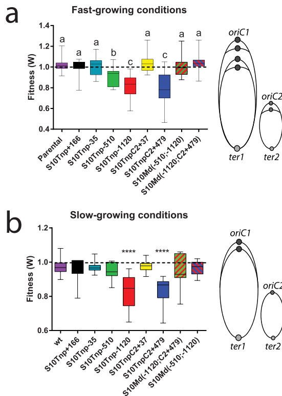
FIG 2 Movant strain fitness in pairwise competition experiments. S10 relocation effect on fitness was assessed by averaging the obtained W values against Parental–1120:: gfpmut3* of the parental, movant, and merodiploid strains. Results are shown in standard box-and-whisker plots showing the medians, minima, and maxima of W values. Statistical significance was analyzed using nonparametric tests and the Dunn test for multiple comparisons of the means obtained for each strain. (a) Competition experiments done under fast-growth conditions when overlapping replication rounds occur as depicted in the right panel. Letters denote groups showing statistically significant differences ( P of at least <0.01 ). (b) Competition experiments performed under slow-growth conditions in the absence of multifork replication as depicted in the right panel. ****, P < 0.0001 . The rest display no statistically significant differences with respect to the parental strain.
