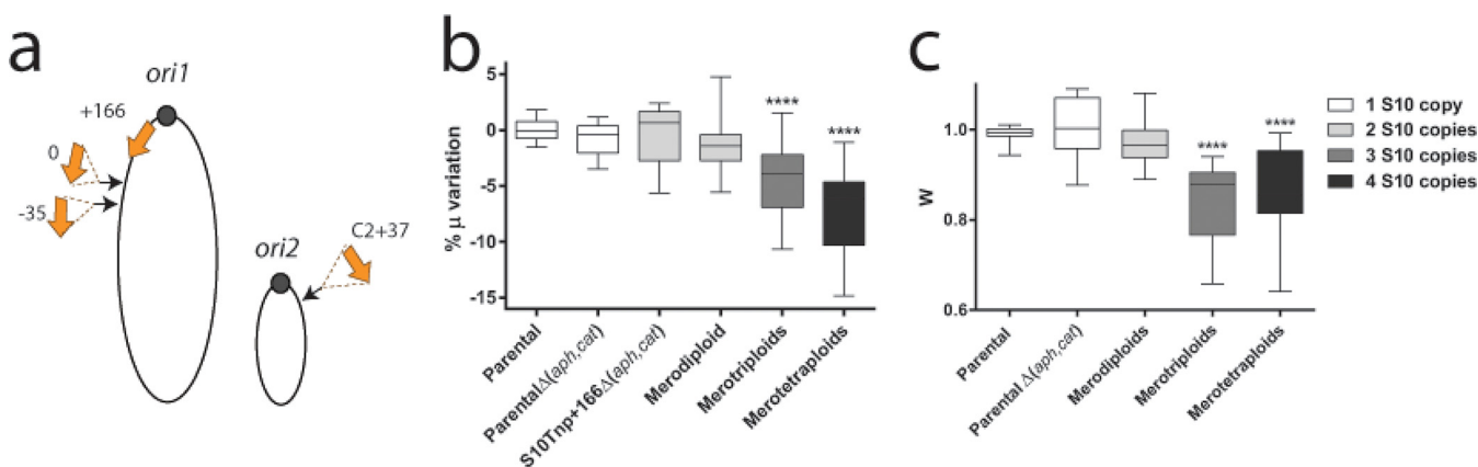
FIG 3 Impact of additional S10 copies in V. cholerae . (a) Several S10 copies (orange arrows) were inserted within the S10Tnp+166 \Delta ( aph, cat ) genome. Their insertion sites, drawn as black arrows and the coordinates (in kilobase pairs from the original location), are shown within V. cholerae chromosomes. (b) The S10 ploidy effect on growth rate was quantified by averaging obtained \mu in at least 3 independent experiments, with 3 or more biological replicates, for each mutant strain and normalizing it to the \mu of the parental strain. Results are expressed as percentage of the variation (% \mu ) with respect to parental strains. (c) Competition experiments done under fast-growth conditions. For panels b and c, data are shown using box-and-whisker plots. Statistical significance was analyzed by a nonparametric test, and the Dunn test was done to compare the mean values obtained for each strain. ****, P < 0.0001 .
