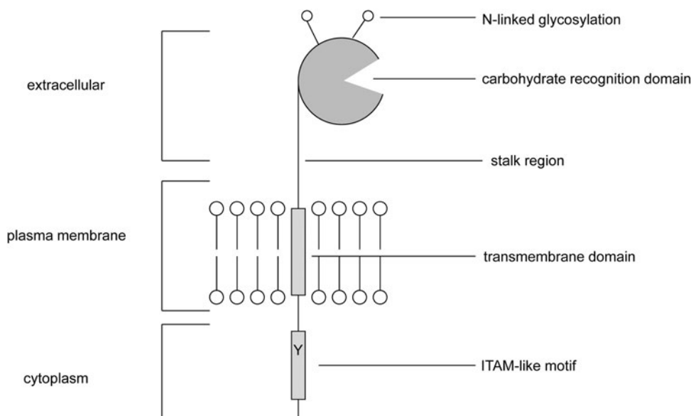
Fig. 1 A schematic representation of the structure of Dectin-1
