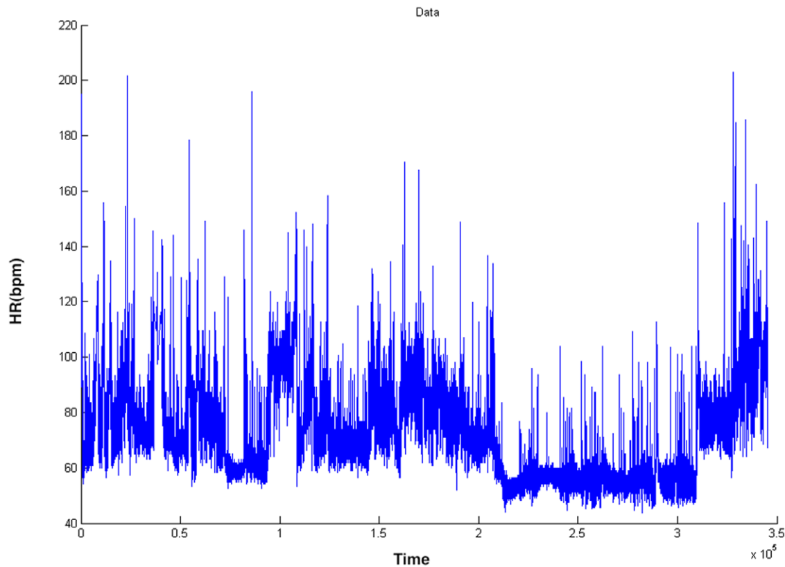
Figure 1. A typical 24 hour heart rate time series. Beats per minutes are shown as a function of time.
