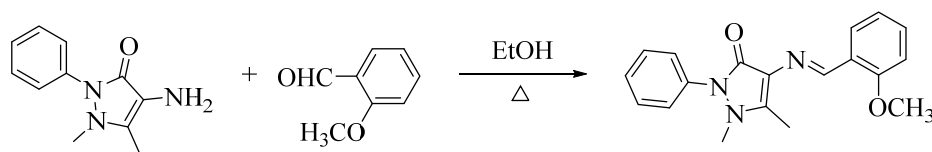
Figure 1: Synthesis of (E)-4-[2-methoxybenzylidene amino]-1,5-dimethyl-2-phenyl-1H-pyrazol-3(2H)-one (MBA-dMPP)
