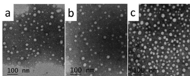
Fig. 3 TEM micrographs of N z -lysine based derivatives solutions with 5 times the CMC: (a) C8, (b) C10, (c) C12.
