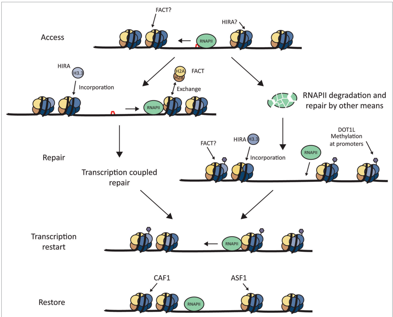
Figure 2. Chromatin remodeling during the transcriptional restart upon DNA damage. This model shows an overview of chromatin remodeling necessary for transcriptional restart after UV damage. When RNAPII is stalled by a lesion, the damaged site has to be made accessible for repair. This is done by chromatin remodelers like NAP1L1, p300, and HMG1 (not shown), which are most likely involved in the reverse translocation of RNAPII. FACT mediates H2A/H2B exchange which might give the chromatin extra plasticity needed for this backtracking. In another scenario, if RNAPII is degraded, other repair mechanisms will remove the damage and in order for transcription to restart new RNAPII has to be loaded onto the DNA. As DOT1L is a histone methyltransferase that prevents heterochromatin spreading and might therefore stimulate loading of new RNAPII after it has been degraded upon DNA damage. Both these pathways could be stimulated by the incorporation of new histone H3.3 by HIRA. DOT1L and FACT might also play a role in either of these events. This chromatin remodeling provides a specific environment stimulating the transcription restart after DNA damage. When transcription rates are recovered, the DNA can be remodeled back to its predamaged state to maintain epigenetic information by for instance CAF1 and ASF1.
