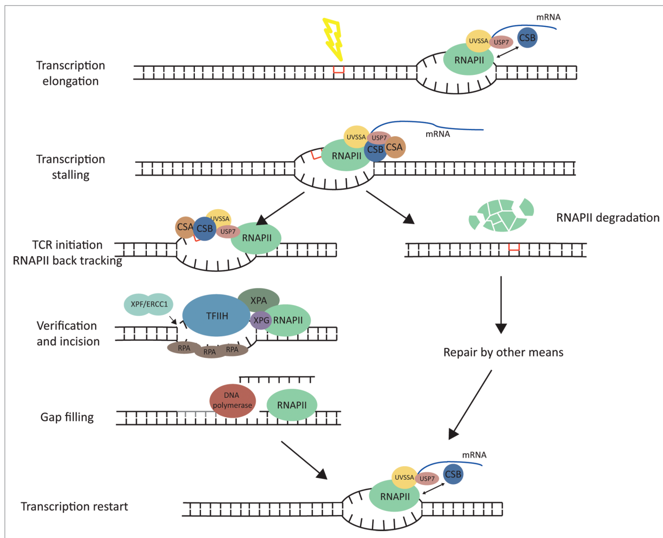
Figure 1. Model of mammalian transcription coupled repair. During transcription UVSSA, USP7, and CSB transiently interacts with RNAPII. When the polymerase encounters a lesion in the DNA, the stalled complex will block access of the repair proteins to the lesion. Therefore, RNAPII has to be either moved back along the DNA to enable TC-NER initiation by CSB, UVSSA, USP7, and CSA (left side) or degraded to allow repair by other repair mechanisms (right side). In TC-NER, the DNA is unwound by TFIIH that together with XPA is responsible for the damage verification. The endonucleases XPF/ERCC1 and XPG are positioned by RPA and cleave the damaged DNA strand and remove about 30 bases around the damage. DNA polymerases fill the single-stranded gap followed by ligation of the nick by DNA ligases I or III to complete the NER reaction. Upon damage removal the transcription need to restart for proper cellular functioning.
