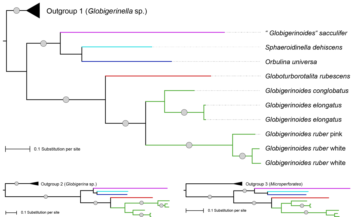
Fig 4. Maximum likelihood phylogeny of representative SSU rDNA sequences of extant species of the genus “ Globigerinoides ” and related taxa. The lower panels show the topology for trees rooted on different outgroups (Table 1). Branches with bootstrap support > 95% (1000 replicates) are marked with grey circles.
