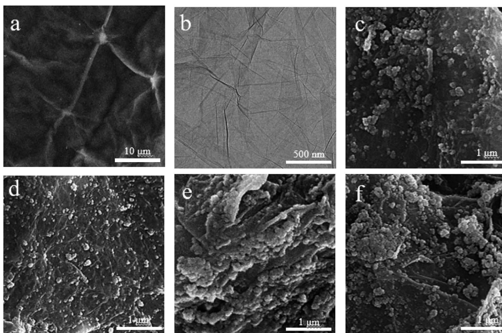
Fig. 7 TEM and SEM images of GO (a and b) and Fe 3 O 4 /GO buckypapers with different m_{\text{Fe}_3\text{O}_4} to m_{\text{GO}} ratios: (c) 8 : 2, (d) 7 : 3, (e) 6 : 4 and (f) 5 : 5.
