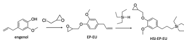
Scheme 1 Synthesis route of Hydrosilylation epoxidized eugenol (HSI-EP-EU).
