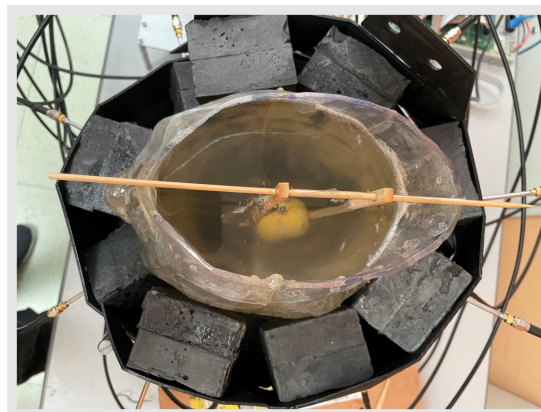
Figure 2. Homogeneous phantom (HP) with immersed stroke target and supporting wooden sticks.
