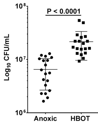
FIG 3 Hyperbaric oxygen treatment (HBOT) effect on bacterial growth in Pseudomonas aeruginosa biofilms. Effect of anoxic (circles) and HBOT (squares) conditions on bacterial growth (calculated as \Delta\log_{10} cell numbers) after treatment for 90 min on agarose-embedded PAO1 biofilms. Bars indicate the mean \pm standard error of the mean (SEM) ( n = 19 ). Statistical significance ( P \leq 0.05 ) was evaluated by the Student's t test.
