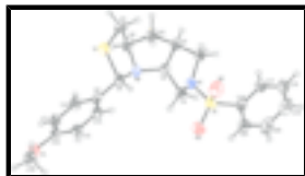
Fig. 1. The molecular structure of the title compound, showing 30% probability displacement ellipsoids.
