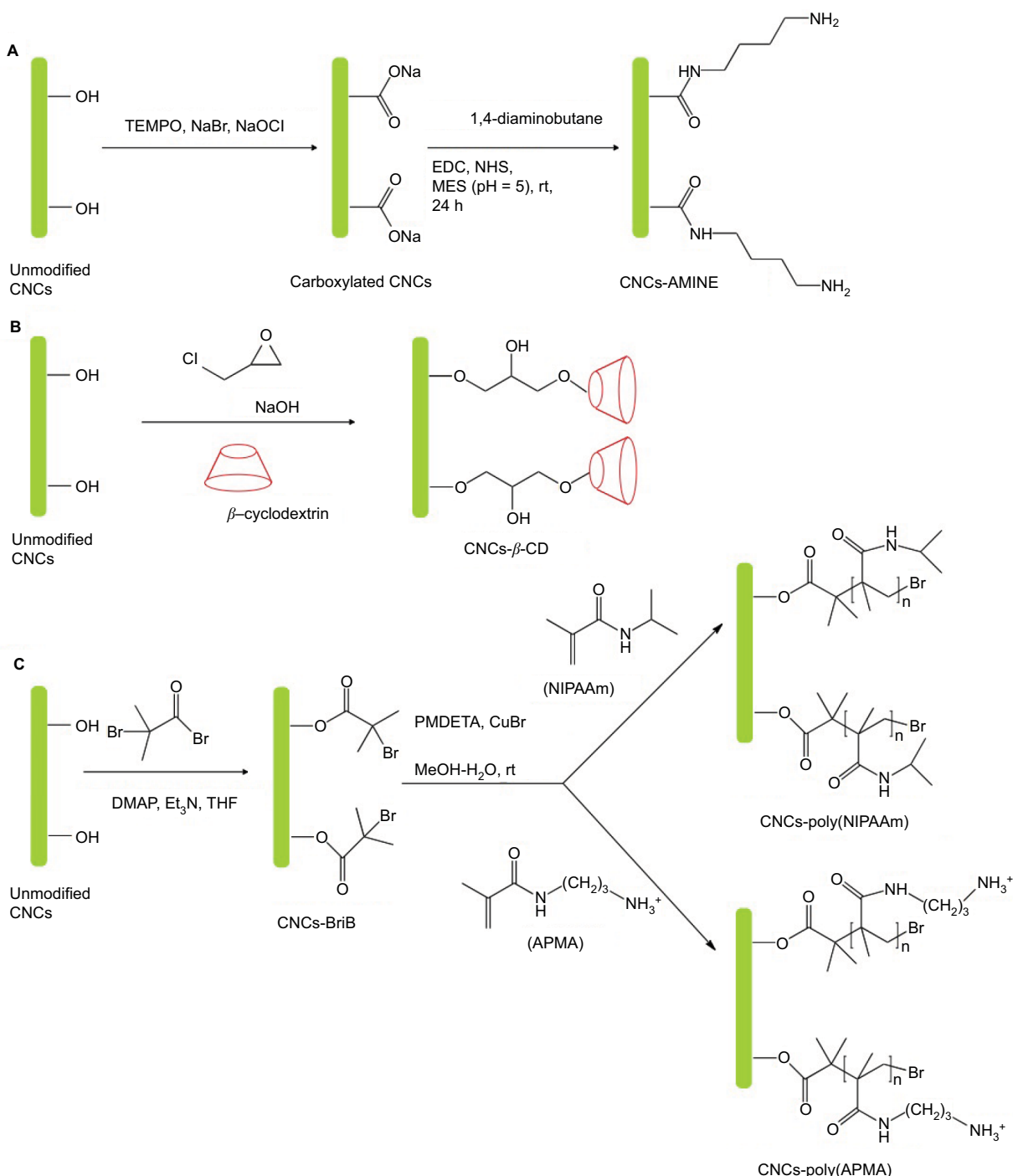
Scheme 1 Synthesis of surface-modified CNCs ( A ) anionic CNCs-AMINE, ( B ) anionic CNCs- \beta -CD, ( C ) anionic CNCs-poly(NIPAAm) and cationic CNCs-poly(APMA). Abbreviations: AMINE, amino-functionalized; CNCs, cellulose nanocrystals; CNCs- \beta -CD, CNCs grafted with \beta -cyclodextrin; poly-(APMA), poly-( N -3-aminopropyl) methacrylamide; poly-(NIPAAm), poly( N -isopropylacrylamide); rt, room temperature; EDC, N-Ethyl-N'-(3-dimethylaminopropyl)carbodiimide; NHS, N-hydroxysuccinimide; MES, 2-( N -Morpholino)ethanesulfonic acid; THF, tetrahydrofuran; DMAP, 4-(Dimethylamino)pyridine; PMDETA, N,N,N',N',N''-pentamethyldiethylenetriamine.
