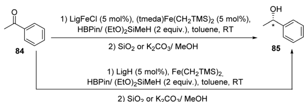
Scheme 19 PdmBOX iron(II) complex catalyzed hydrosilylation of acetophenone.
