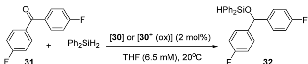
Scheme 8 Hydrosilylation of 4,4'-difluorobenzophenone by neutral or in situ -oxidised analogue of the catalyst.
