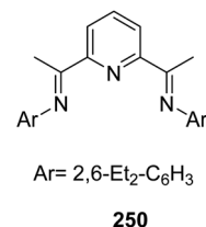
Fig. 10 Bis-(imino)pyridine ligand.
