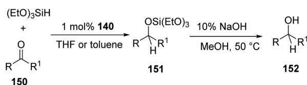
Scheme 31 Ketone hydrosilylation using 2,6- [[\text{(Pr)}_2\text{PO}]_2\text{C}_6\text{H}_3]\text{Fe}(\text{H})(\text{PMe}_3)_2 .
