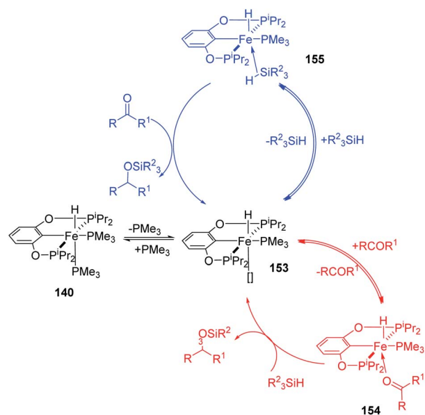
Scheme 32 Possible mechanistic pathways for carbonyl hydrosilylation catalyzed by 2,6- [[\text{(Pr)}_2\text{PO}]_2\text{C}_6\text{H}_3]\text{Fe}(\text{H})(\text{PMe}_3)_2 . Adapted with permission from ref. 59. Copyright 2011 American Chemical Society.
