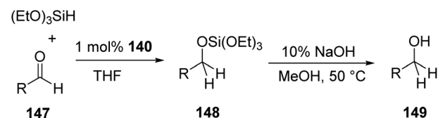
Scheme 30 Aldehyde hydrosilylation using 2,6-((( i Pr) 2 PO) 2 C 6 H 3 SiFe(H)(PMe 3 ) 2 .
