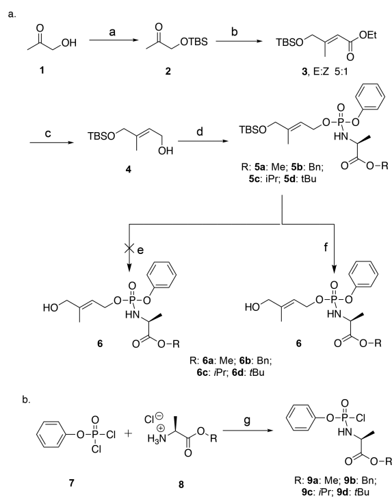
Scheme 1. (a) Synthesis of HMBP ProPAGens and (b) Synthesis of Aryl Phosphorochloridates 29
