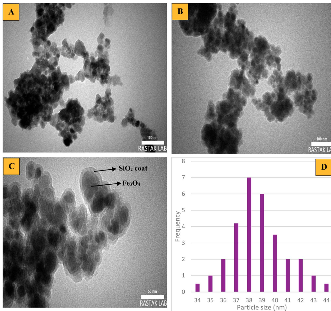
Fig. 6 TEM images of (A) \text{Fe}_3\text{O}_4 , (B and C) mesalamine/GPTMS@ \text{SiO}_2 @ \text{Fe}_3\text{O}_4 , and (D) a histogram of mesalamine/GPTMS@ \text{SiO}_2 @ \text{Fe}_3\text{O}_4 .
