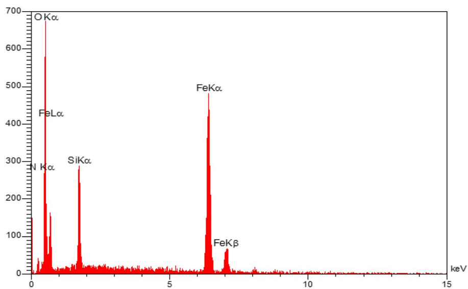
Fig. 7 EDX spectra of mesalamine/GPTMS@ \text{SiO}_2 @ \text{Fe}_3\text{O}_4 .
