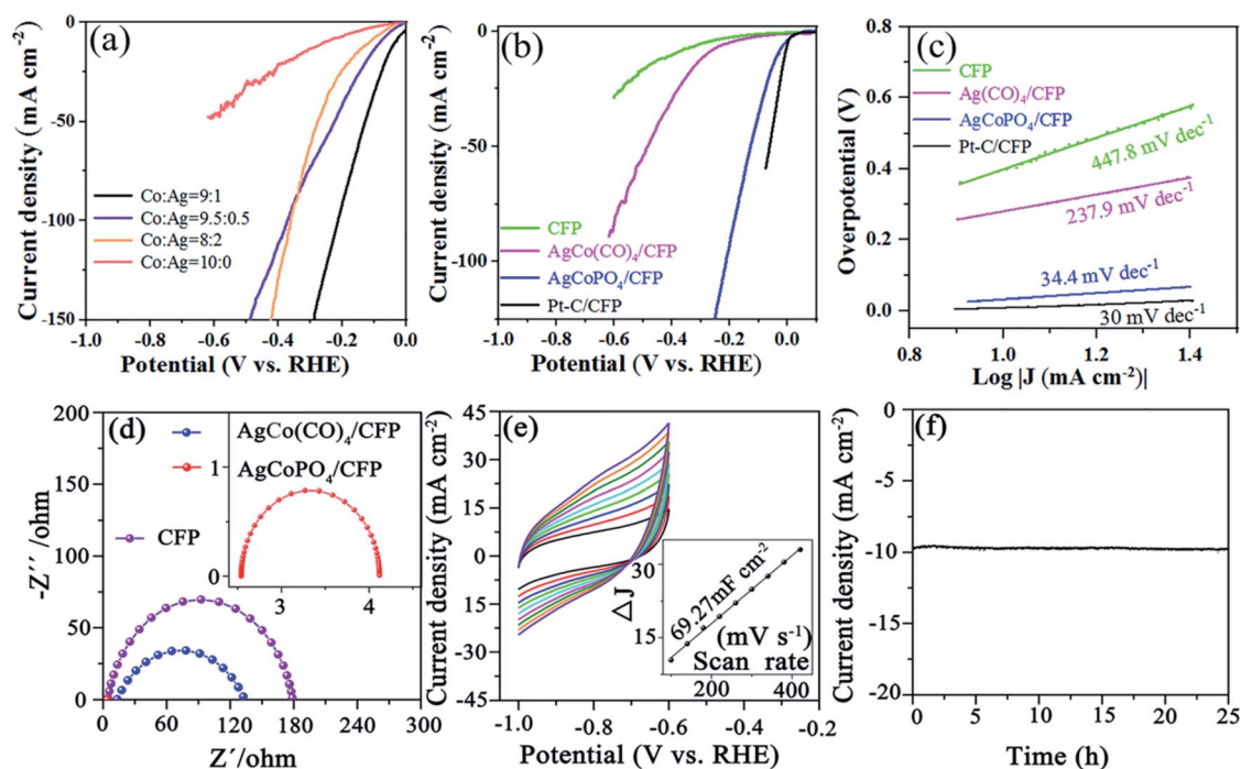
Fig. 3 (a) Hydrogen evolution reaction (HER) properties: polarization curves for Co : Ag/CFP (Co : Ag = 9 : 1, 9.5 : 0.5, 8 : 2, 10 : 0) in 1 M NaOH with a scan rate of 5 \text{ mV s}^{-1} . (b) Polarization curves without iR compensation for \text{AgCoPO}_4/\text{CFP} and \text{AgCo}(\text{CO})_4/\text{CFP} and Pt-C/CFP. (c) Tafel plot extracted from the corresponding polarization curves with iR compensation. (d) Nyquist plots of the \text{AgCo}(\text{CO})_4/\text{CFP} and CFP with an applied bias of 0.4 V, inset is \text{AgCoPO}_4/\text{CFP} . (e) Cyclic voltammetry (CV) scans for \text{AgCoPO}_4/\text{CFP} nanorod structure in 1 M NaOH and capacitive current at -0.8 \text{ V} as a function of the scan rate. (f) I-t curves of \text{AgCoPO}_4/\text{CFP} for 25 h at -0.032 \text{ V} in the cathode.
