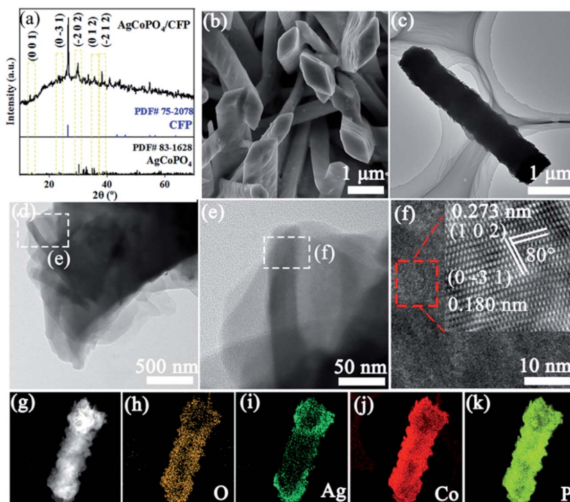
Fig. 2 (a) XRD patterns of \text{AgCoPO}_4/\text{CFP} . (b) SEM images of \text{AgCoPO}_4/\text{CFP} . (c–e) TEM images at different magnifications. (f) HRTEM micrograph. (g–k) Energy dispersive X-ray spectroscopy (EDS) elemental mapping of O (orange) (h), Ag (green) (i), Co (red) (j), and P (chartreuse) (k).
