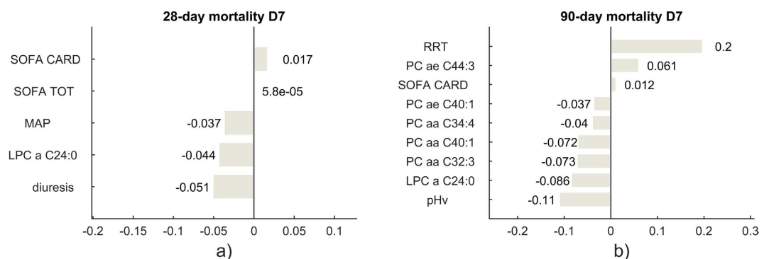
Figure 5. Elastic Net coefficients built on metabolites concentration and clinical parameters collected at day 7 for 28-day (a) and 90 days mortality (b). The MSE computed for the models are 0.23 for the 28-day one (a) and 0.24 for the 90-day (b). SOFA CARD: cardiovascular SOFA score; SOFA TOT: total SOFA score; MAP: mean arterial pressure; pHv: venous pH; diuresis (ml/die) collected at day 7; RRT: renal replacement therapy administered during the first 7 days of treatment.
